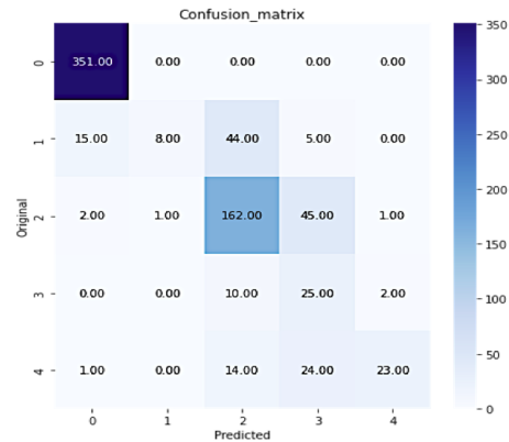
Figure 13. Confusion matrix ResNet50
