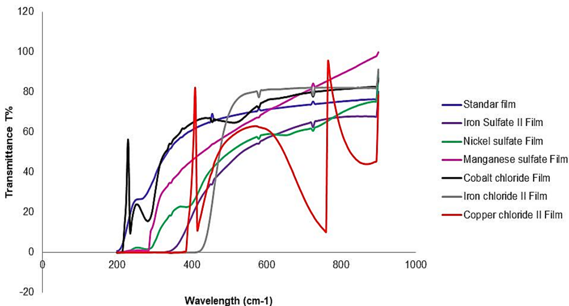
Figure 3. UV-Vis light transmittance rate in arrowroot films incorporating different metals. Source: Authors, 2021.
